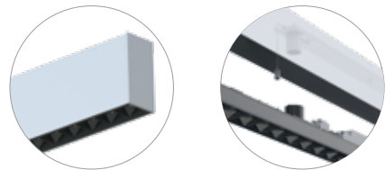
Micro reflector design UGR<10 Push-in and push-out structure, easy for installation and maintenance
