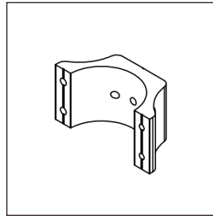
bracket 90*45*39mm
